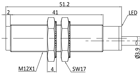
Fig. 1 Inductive sensor with cable (flush)
