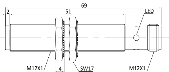
Fig. 5 Inductive sensor with M12 connector (flush)
