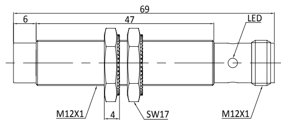
Fig. 6 Inductive sensor with M12 connector (non-flush)
