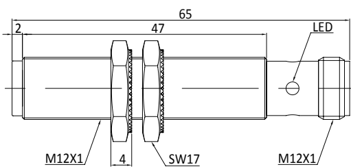
Fig. 7 Inductive sensor with M12 connector (flush)
